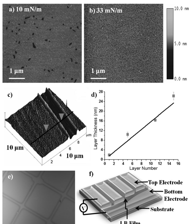
Figure 3. a, b) Surface morphology of the LB monolayers for \mathbf{1}^{\text{I}} at 10 \text{ mN m}^{-1} (a) and at 33 \text{ mN m}^{-1} (b). c) 3D view of an AFM image of a 15-layer film. d) Layer thickness (nm) versus the number of layers; \mathbf{1}^{\text{I}} (■). e) Optical micrograph of the device; image size = 1240 \times 930 \mu\text{m}^2 . f) Device layout.
