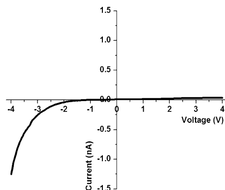
Figure 4. I – V diagram for complex \mathbf{1}^{\text{I}} (—) from 4 to -4 \text{ V} .
